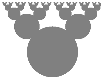
Figure C.4: A recursive shape we call “Mickey Moose”.
